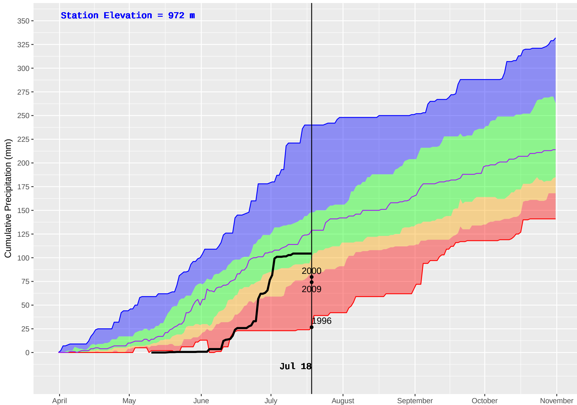
SPARKS LAKE (305) : Historical (1991–2016) and Current (2018) Daily Cumulative Precipitation
